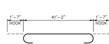
H3 #11 x 44'-4"
