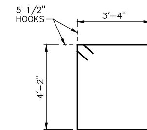
S1 #5 x 15'-11"
